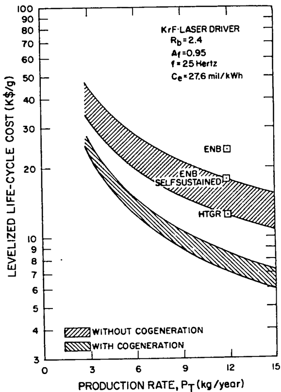
Fig. 4. Unit production cost with the KrF-laser driver.
