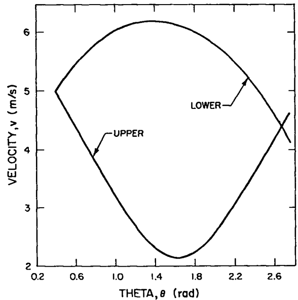
Fig. 11. Protective-layer velocity distribution for the injection velocity of 5 m/s.
